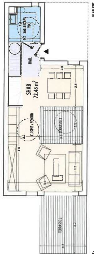
PLAN R+1
