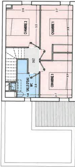
PLAN R+1
