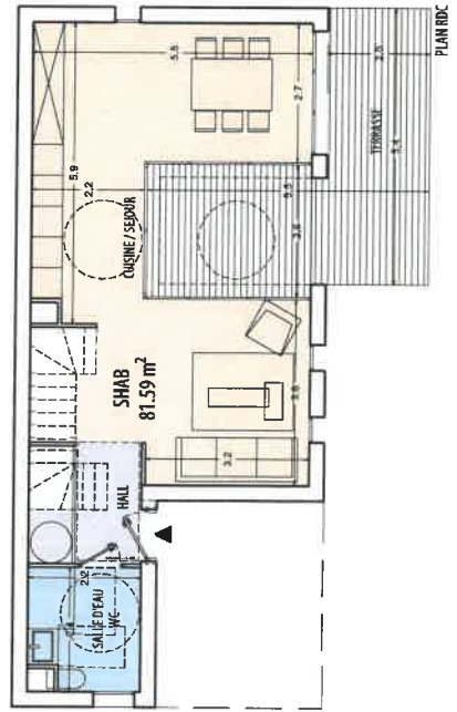
PLAN R+1
