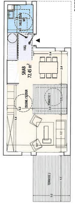
PLAN R+1
