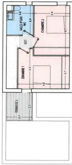
PLAN R+1
