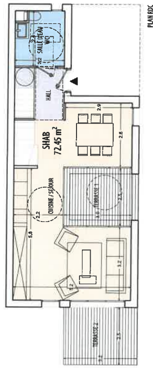
PLAN R+1
